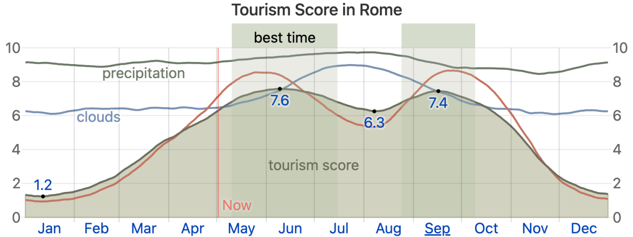
The tourism score (filled area), and its constituents: the temperature score (red line), the cloud cover score (blue line), and the precipitation score (green line).
